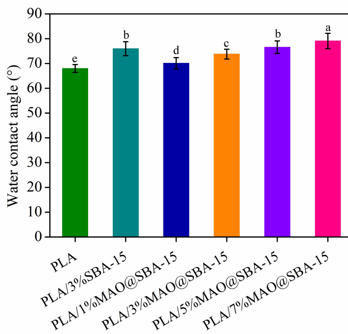
Supplementary Figure 2. Water contact angle of the PLA-based packaging films. Different letters represent statistically significant differences ( P < 0.05 ).
