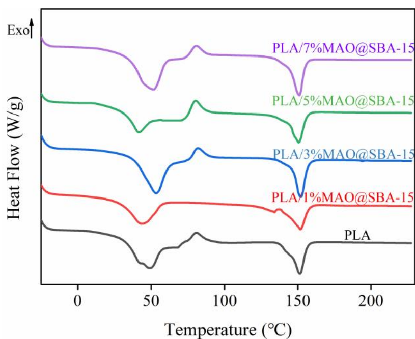
Supplementary Figure 1. DSC curves of the PLA-based packaging films.
